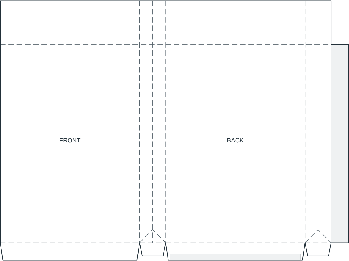
Four-panel gusseted paper pouch
